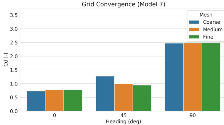
FIGURE 5 RESULTS OF GRID CONVERGENCE STUDY
