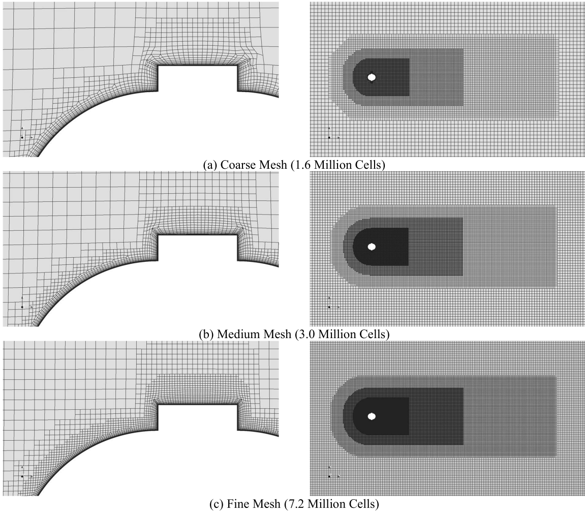
FIGURE 3 THREE SETS OF MESHES FOR GRID CONVERGENCE STUDY
