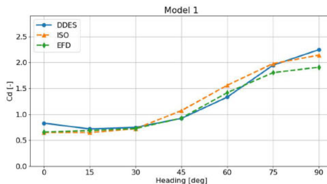
FIGURE 10 DRAG COEFFICIENTS FOR CHORD MODEL1 AT VARIOUS HEADING ANGLES
