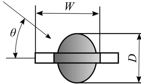
FIGURE 1 GEOMETRY OF A TYPICAL SPLIT TUBE CHORD
