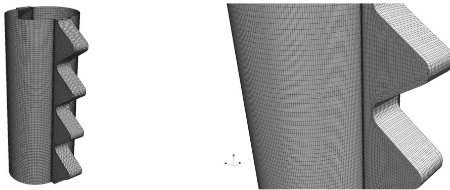
FIGURE 4 SURFACE MESH OF SPLIT-TUBE CHORD (COARSE MESH)
